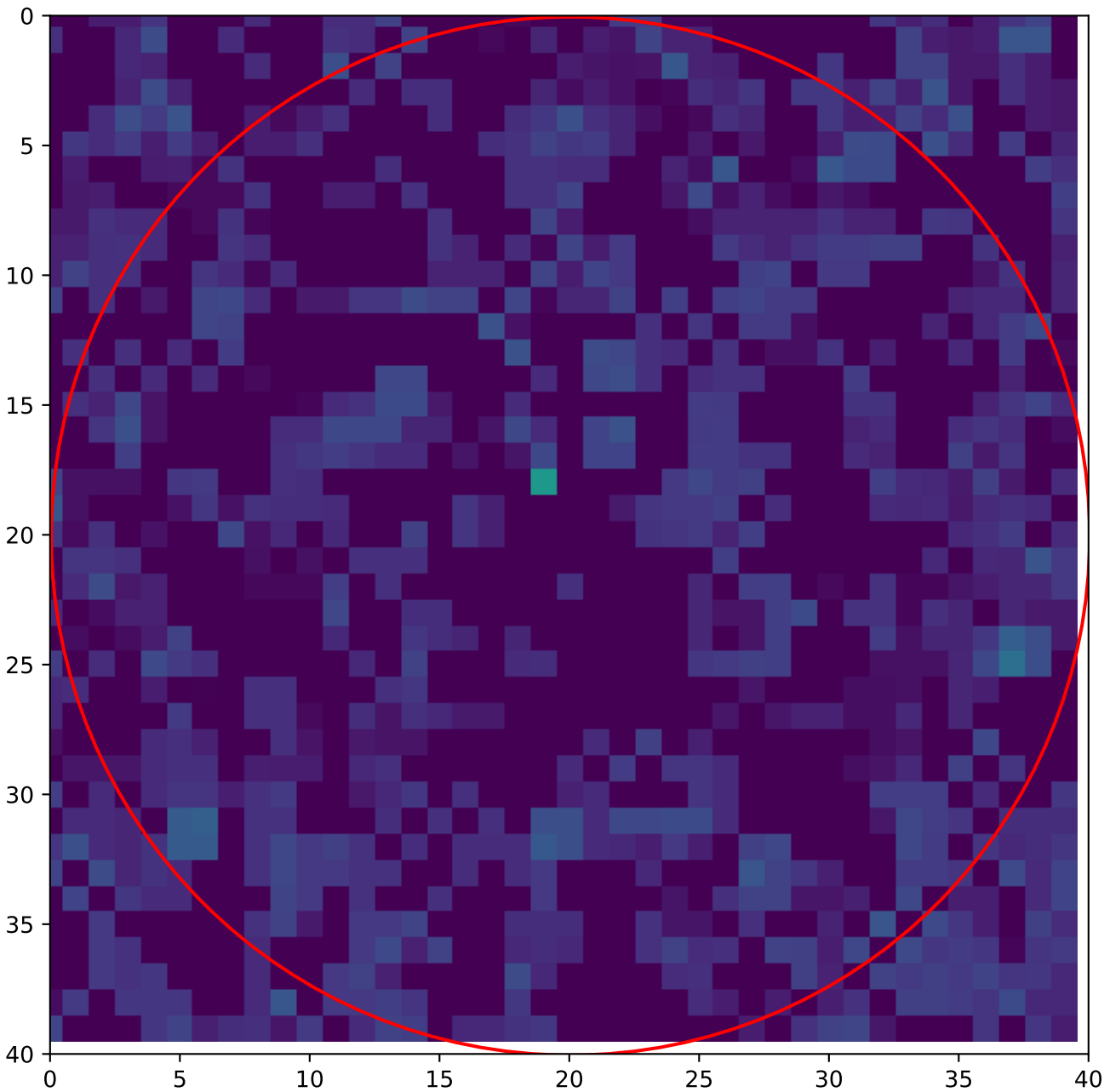
A1 — global hotspot 72 — Annealing 150 °C, 25 h T = 20 °C, v_over = 5 V
