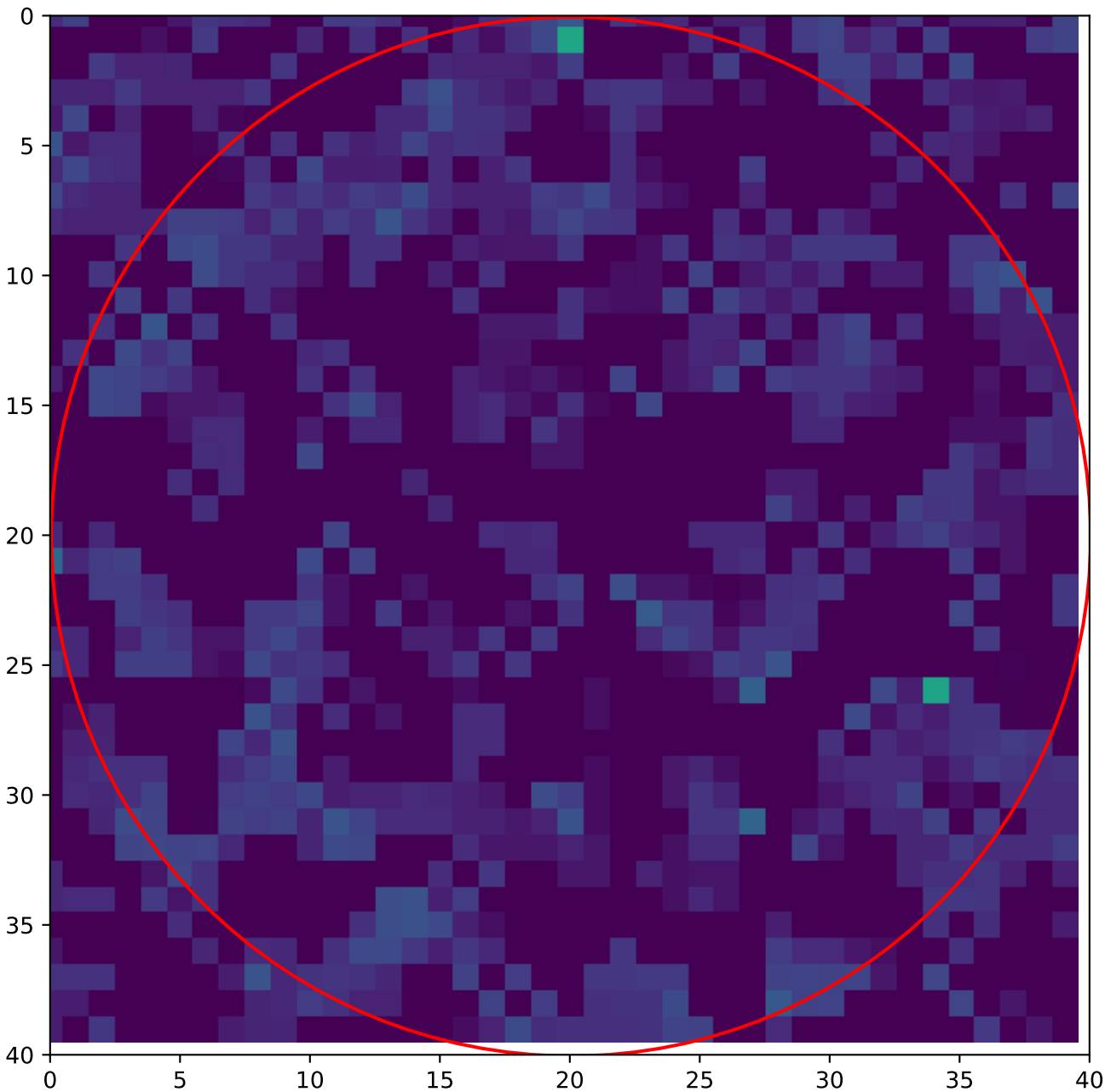
A1 — global hotspot 72 — Annealing 150 °C, 5 h T = 20 °C, v over = 5 V
