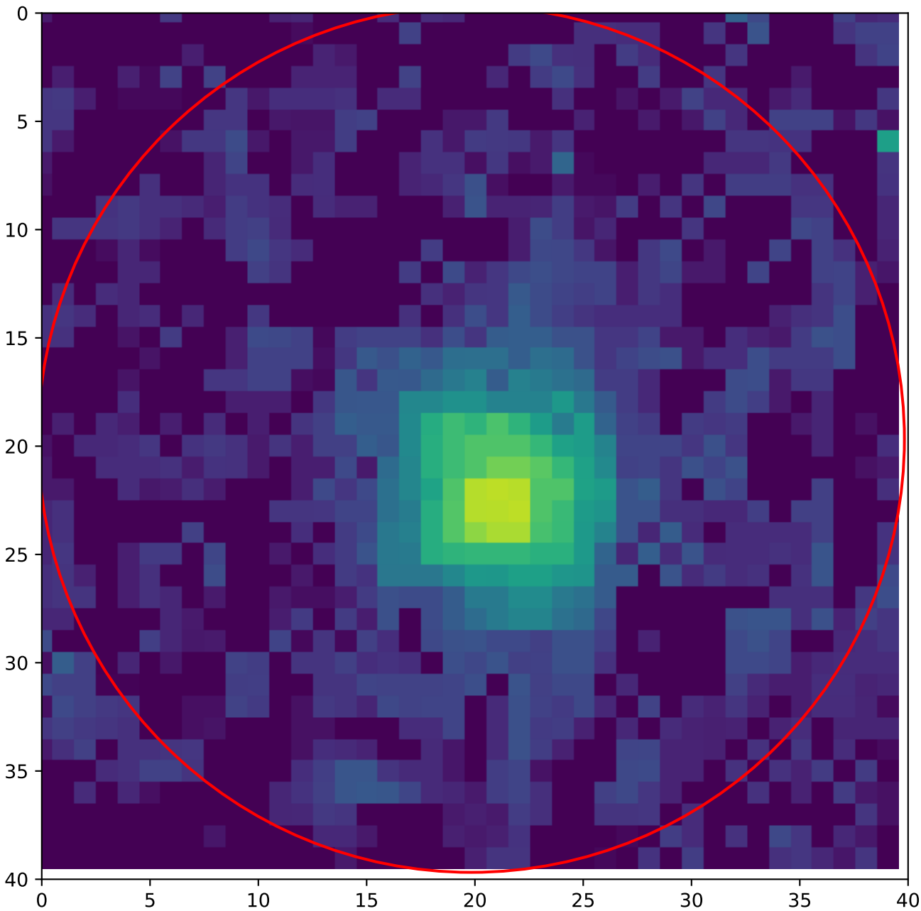
A1 — global hotspot 72 — Annealing 75 °C, 5 h T = 20 °C, v over = 5 V
