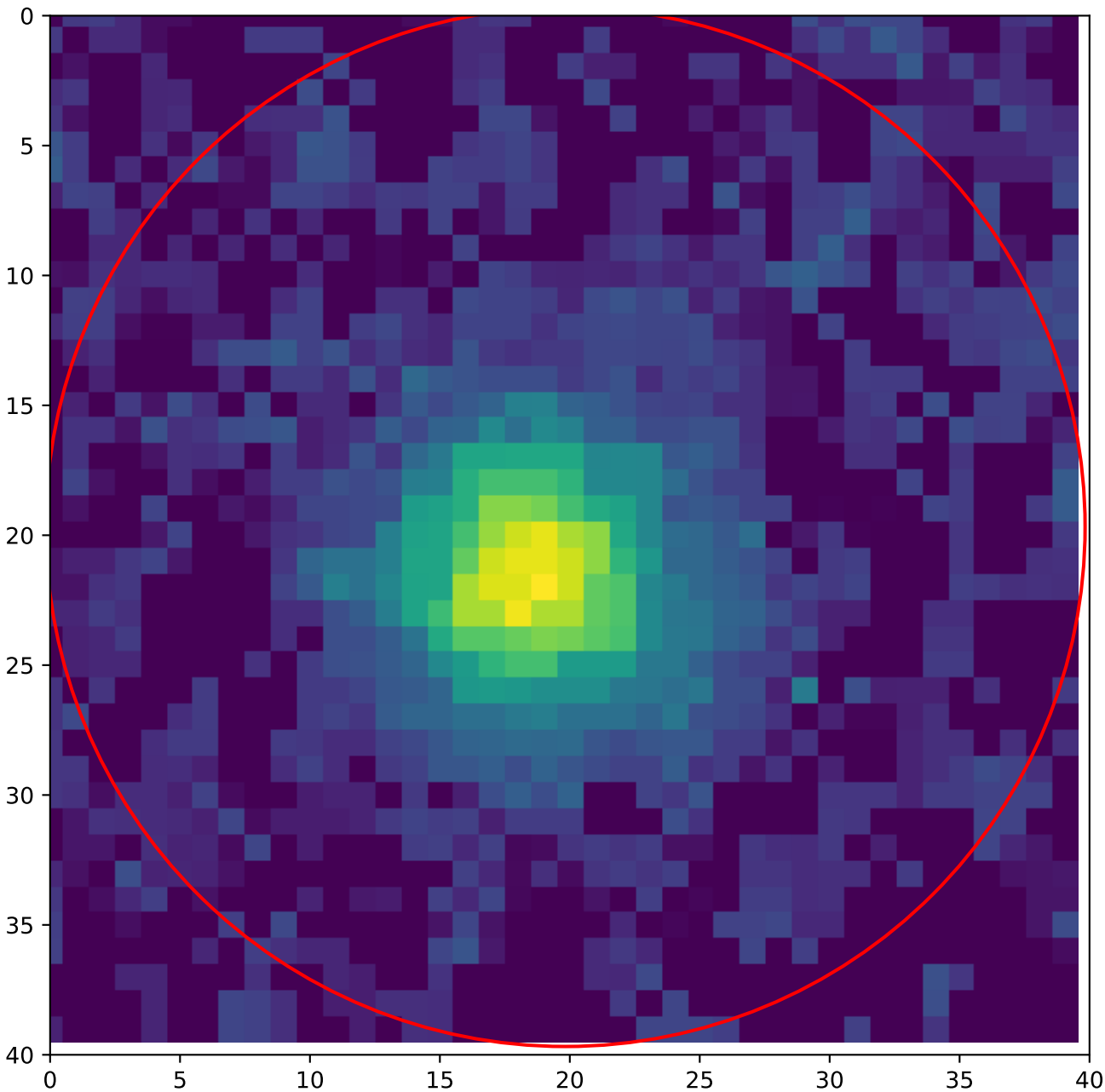
A1 — global hotspot 72 — Before annealing T = 20\text{ }^{\circ}\text{C} , v_{\text{over}} = 5\text{ V}
