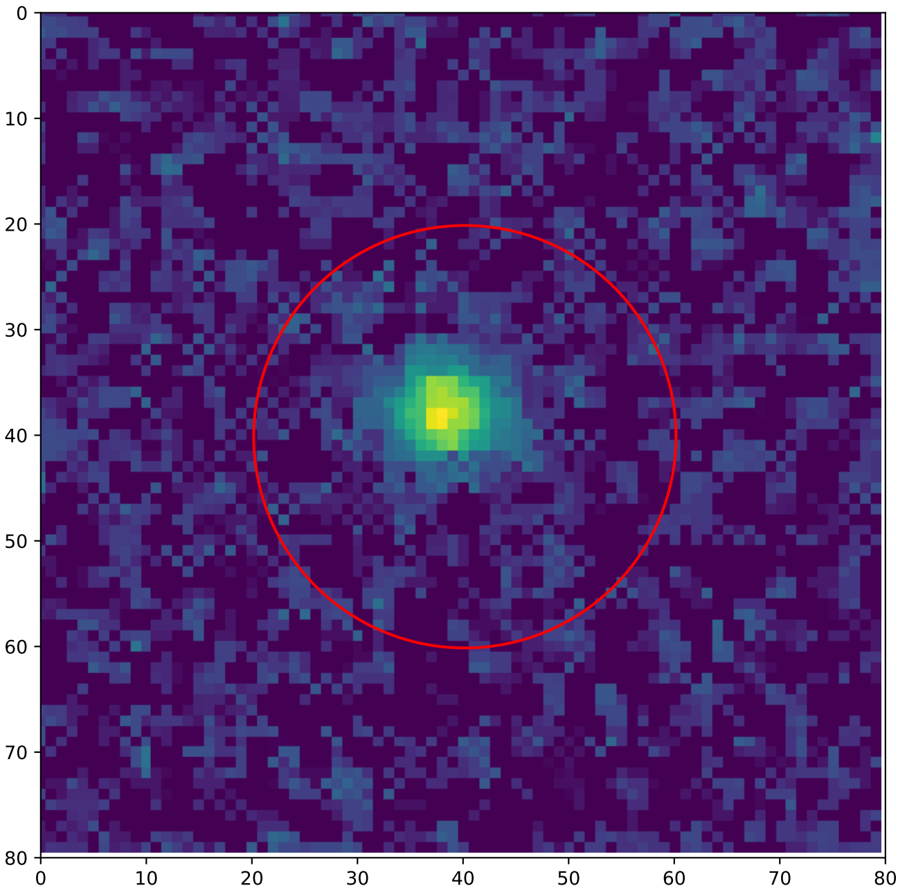
A1 — global hotspot 78 — Annealing 100 °C, 5 h T = 20 °C, v_{\text{over}} = 5 V
