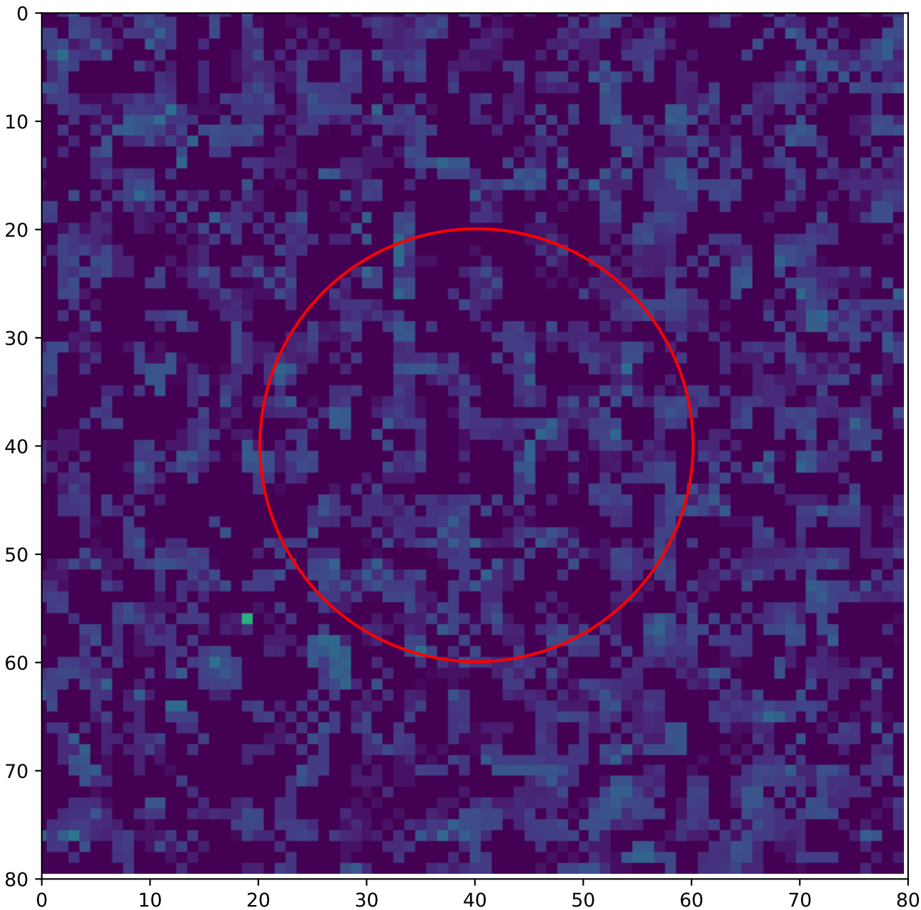
A1 — global hotspot 78 — Annealing 125 °C, 25 h T = 20 °C, v_{\text{over}} = 5 V
