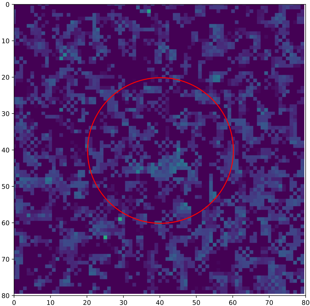
A1 — global hotspot 78 — Annealing 75 °C, 25 h T = 20 °C, v over = 5 V
