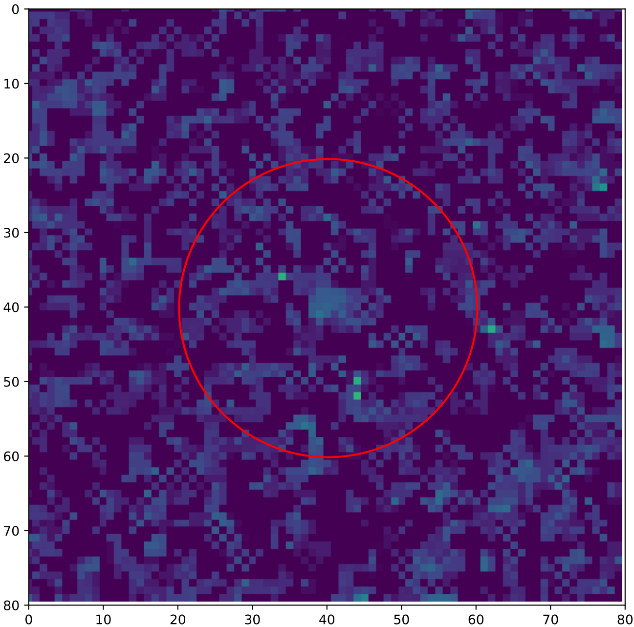
A1 — global hotspot 78 — Before annealing T = 20\text{ }^{\circ}\text{C} , v_{\text{over}} = 5\text{ V}
