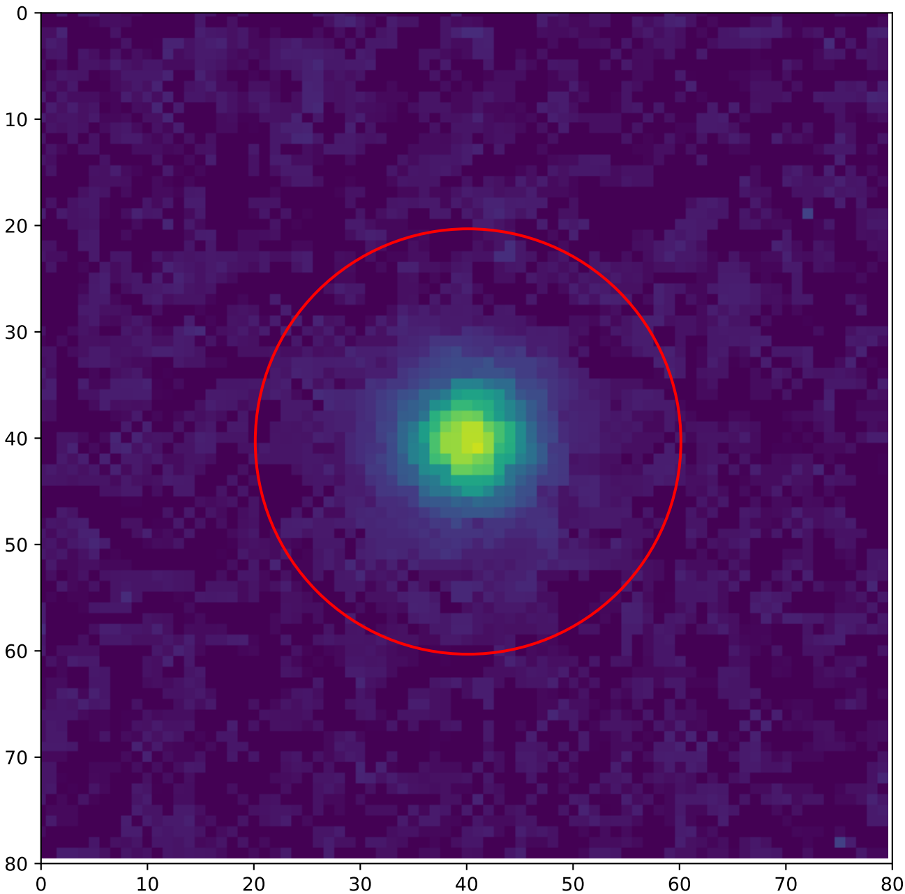
A1 — global hotspot 13 — Before annealing T = 19\text{ }^{\circ}\text{C} , v_{\text{over}} = 5\text{ V}
