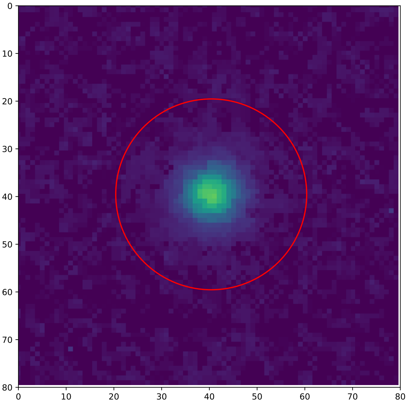
A1 — global hotspot 13 — Before annealing T = 20\text{ }^{\circ}\text{C} , v_{\text{over}} = 5\text{ V}
