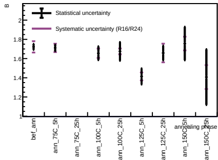
Sensor A1, T = 20 C - Spot 22
