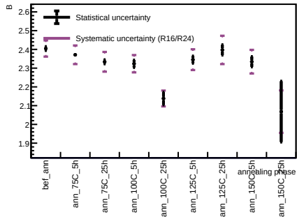
Sensor A1, T = 20 C - Spot 18
