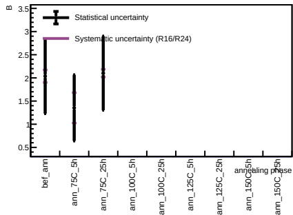
Sensor A1, T = 20 C - Spot 21
