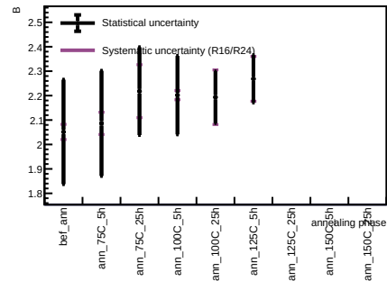
Sensor A1, T = 20 C - Spot 23
