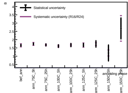
Sensor A1, T = 20 C - Spot 56
