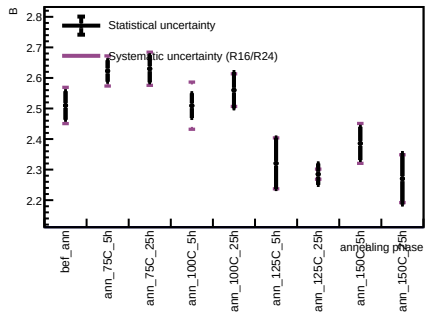
Sensor A1, T = 20 C - Spot 57
