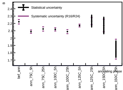
Sensor A1, T = 20 C - Spot 54
