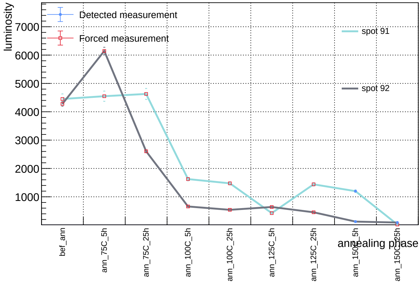
Sensor A1, T = 20 C, v_{\text{over}} = 7 \text{ V} - luminosity vs phase - order 10^3
