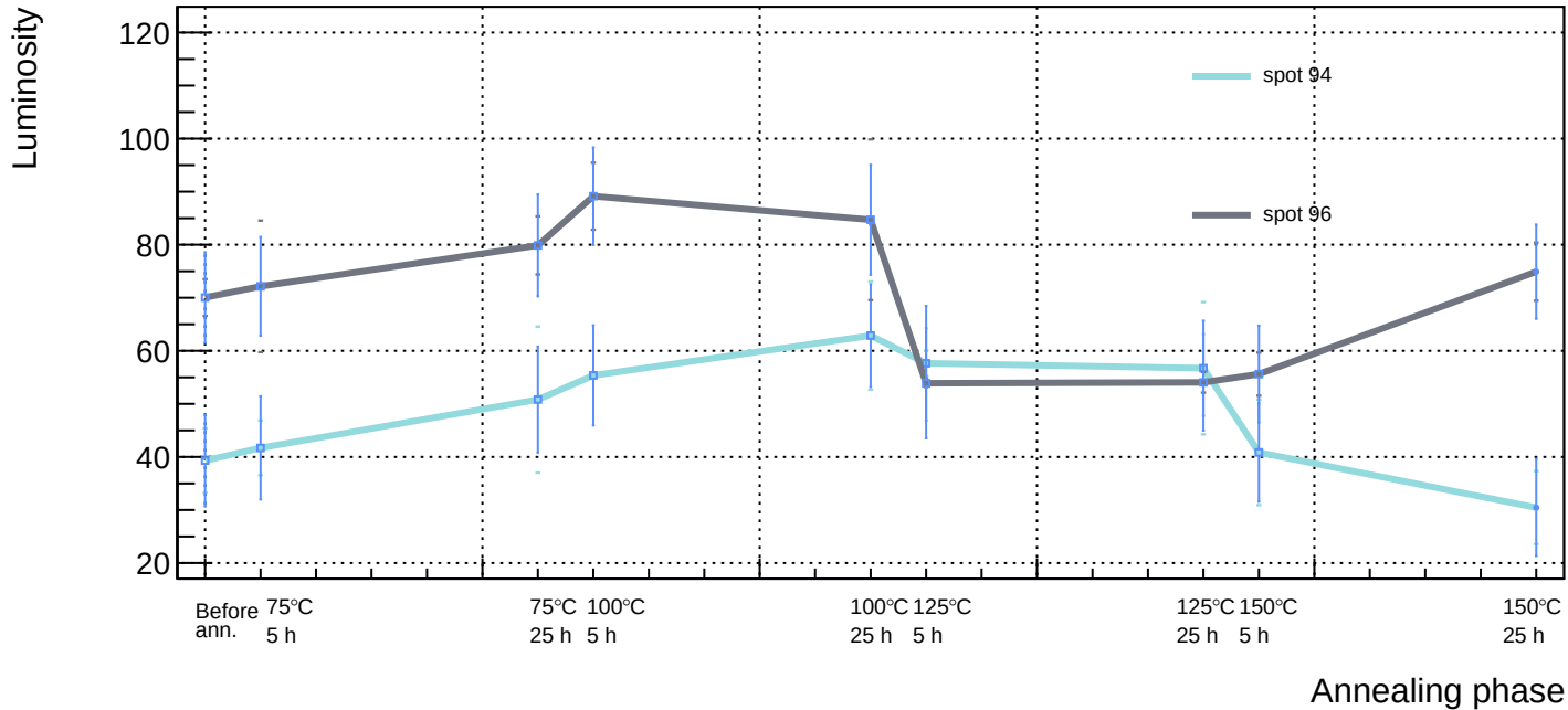
Sensor A1, T = 20\text{ C} , v_{\text{over}} = 7\text{ V} - Approximately constant hotspots
