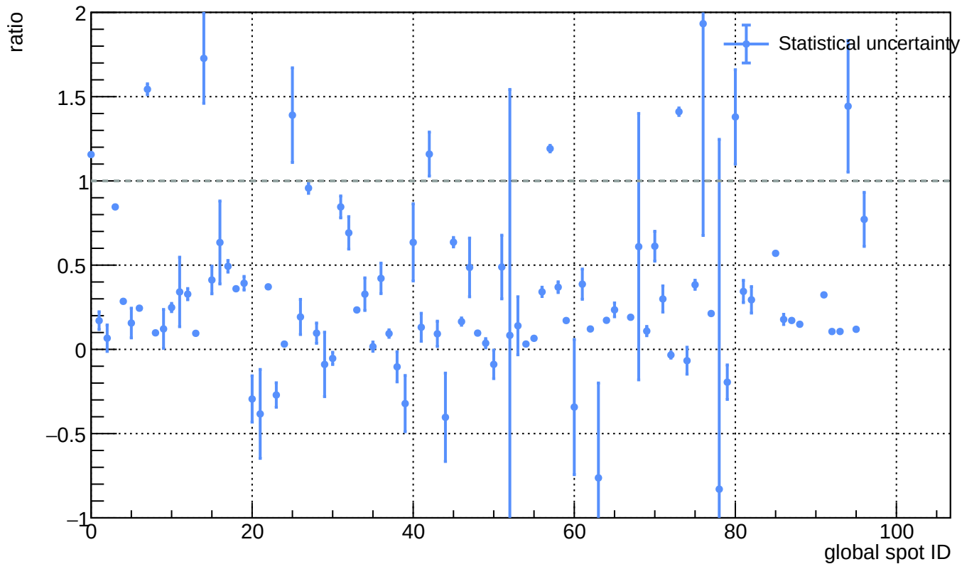
Sensor A1, T = 20 C - L(\text{ann\_125C\_25h}) / L(\text{before\_annealing})
