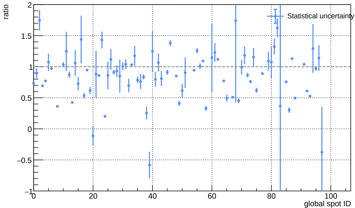
Sensor A1, T = 20 C - L(ann_75C_25h) / L(before_annealing)
