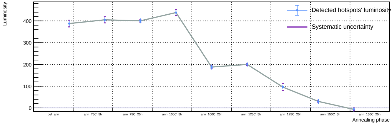
Sensor A1, T = 20\text{ C} , v_{\text{over}} = 7\text{ V} - Spot 10: luminosity vs phase
