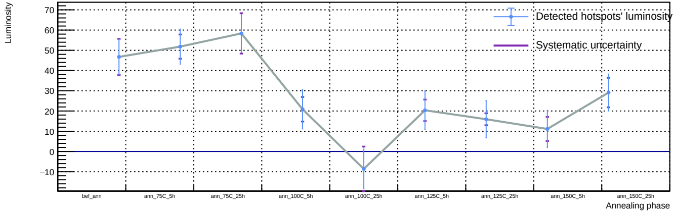
Sensor A1, T = 20\text{ C} , v_{\text{over}} = 7\text{ V} - Spot 11: luminosity vs phase
