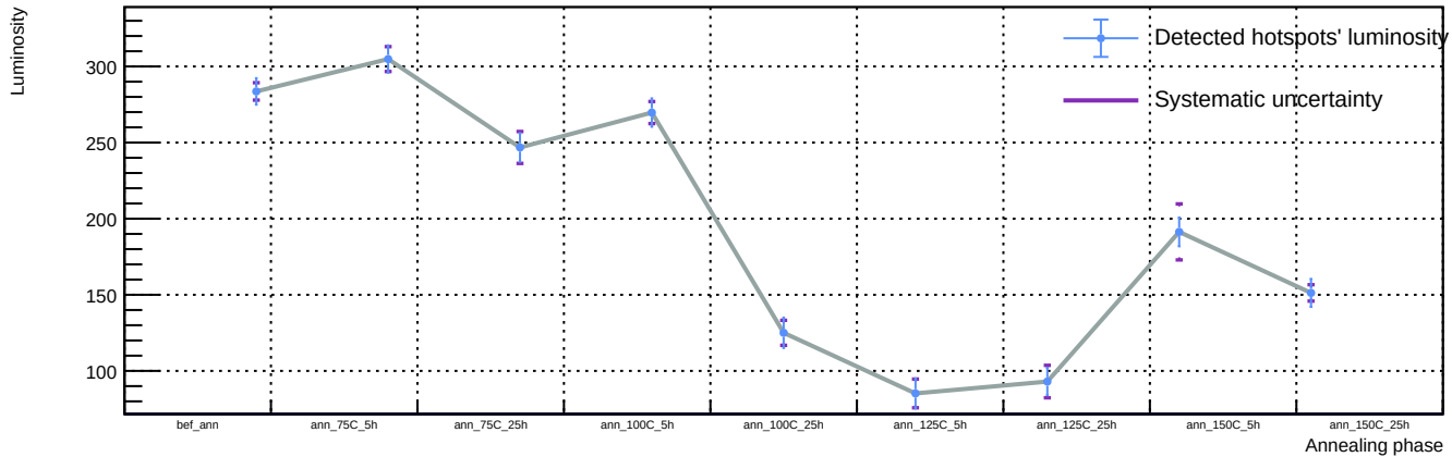
Sensor A1, T = 20\text{ C} , v_{\text{over}} = 7\text{ V} - Spot 12: luminosity vs phase
