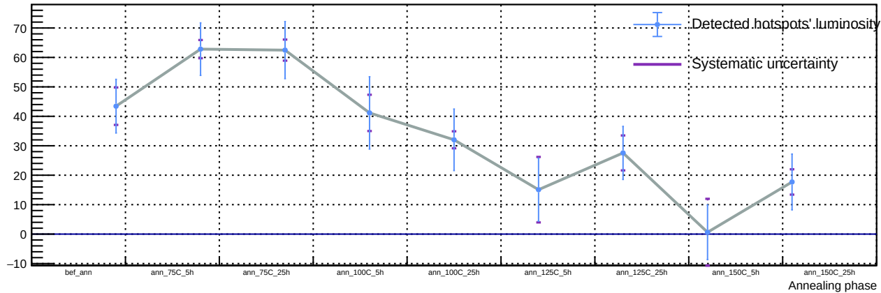
Sensor A1, T = 20\text{ C} , v_{\text{over}} = 7\text{ V} - Spot 16: luminosity vs phase
