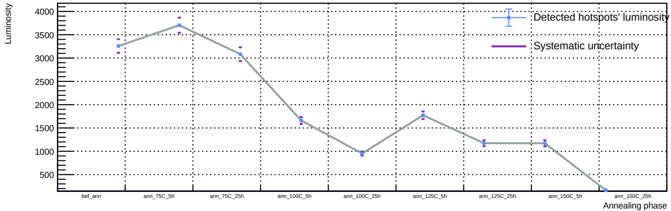
Sensor A1, T = 20\text{ C} , v_{\text{over}} = 7\text{ V} - Spot 18: luminosity vs phase
