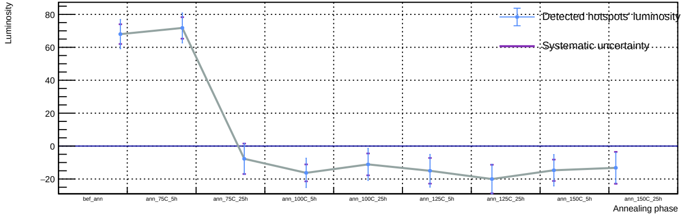
Sensor A1, T = 20\text{ C} , v_{\text{over}} = 7\text{ V} - Spot 20: luminosity vs phase
