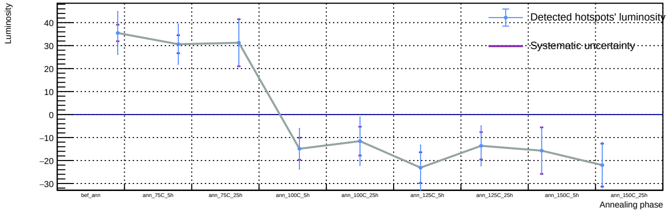
Sensor A1, T = 20\text{ C} , v_{\text{over}} = 7\text{ V} - Spot 21: luminosity vs phase
