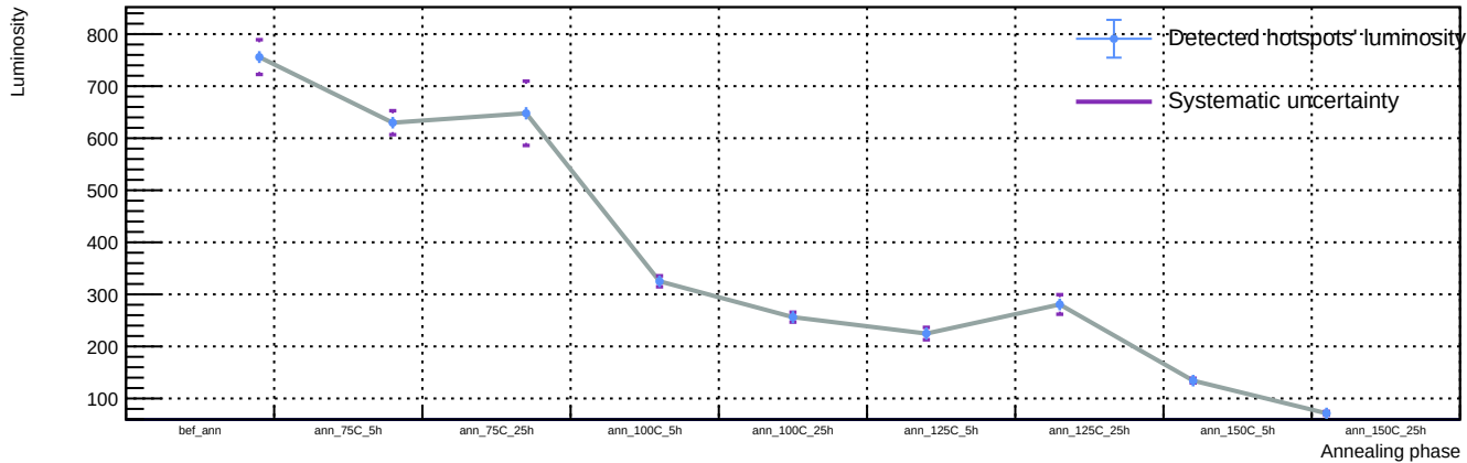
Sensor A1, T = 20\text{ C} , v_{\text{over}} = 7\text{ V} - Spot 22: luminosity vs phase
