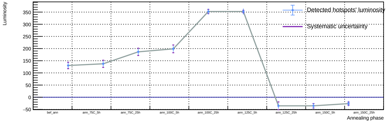
Sensor A1, T = 20\text{ C} , v_{\text{over}} = 7\text{ V} - Spot 23: luminosity vs phase
