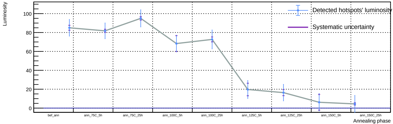
Sensor A1, T = 20\text{ C} , v_{\text{over}} = 7\text{ V} - Spot 26: luminosity vs phase
