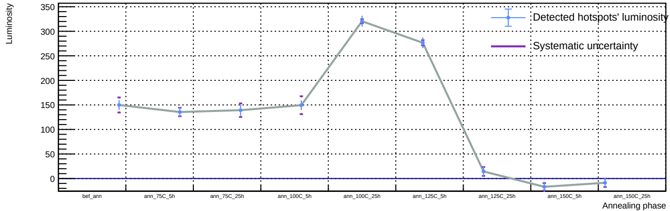
Sensor A1, T = 20\text{ C} , v_{\text{over}} = 7\text{ V} - Spot 28: luminosity vs phase
