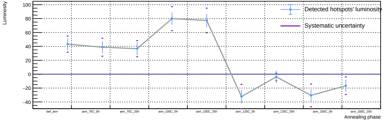
Sensor A1, T = 20\text{ C} , v_{\text{over}} = 7\text{ V} - Spot 29: luminosity vs phase
