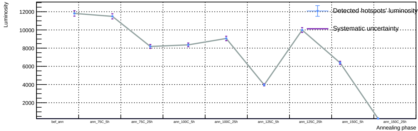
Sensor A1, T = 20\text{ C} , v_{\text{over}} = 7\text{ V} - Spot 3: luminosity vs phase
