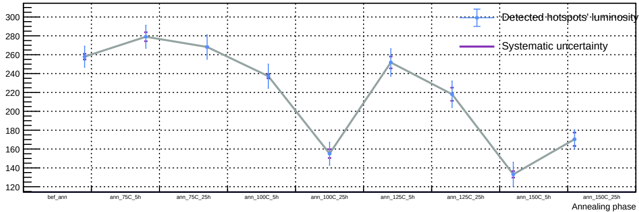
Sensor A1, T = 20\text{ C} , v_{\text{over}} = 7\text{ V} - Spot 31: luminosity vs phase
