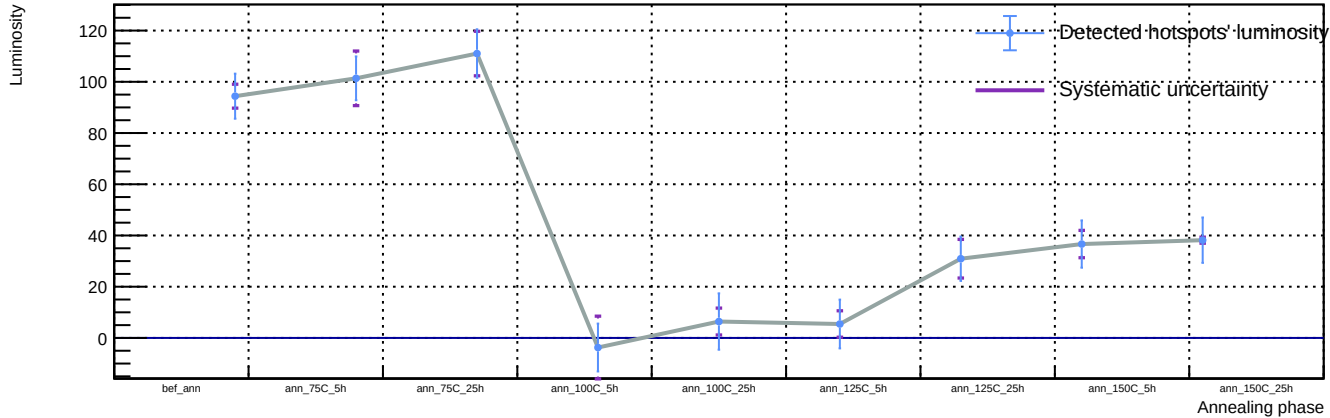
Sensor A1, T = 20\text{ C} , v_{\text{over}} = 7\text{ V} - Spot 34: luminosity vs phase
