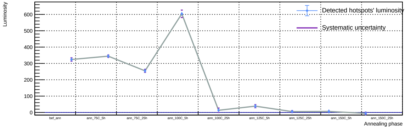
Sensor A1, T = 20\text{ C} , v_{\text{over}} = 7\text{ V} - Spot 35: luminosity vs phase
