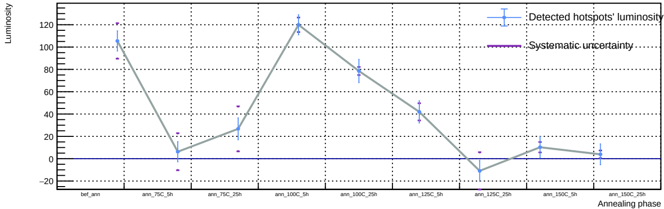
Sensor A1, T = 20\text{ C} , v_{\text{over}} = 7\text{ V} - Spot 38: luminosity vs phase
