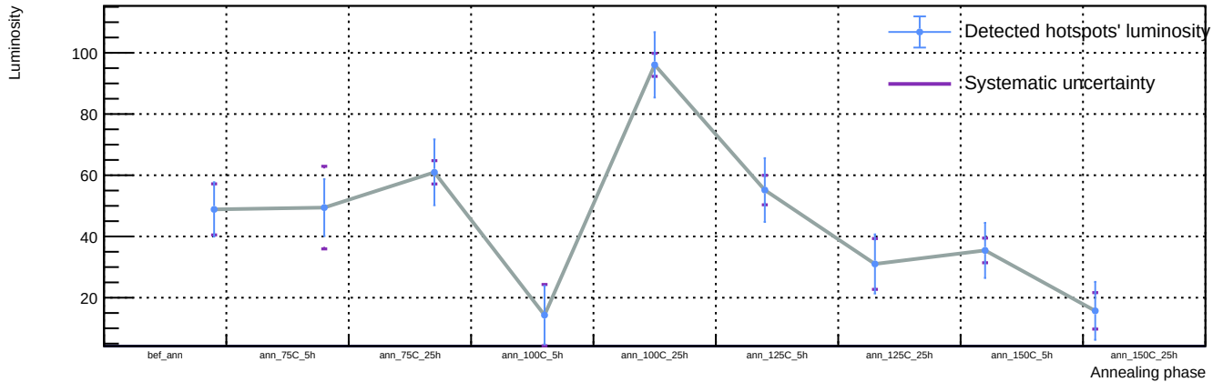
Sensor A1, T = 20\text{ C} , v_{\text{over}} = 7\text{ V} - Spot 40: luminosity vs phase
