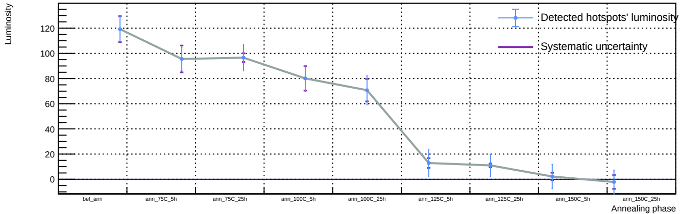
Sensor A1, T = 20\text{ C} , v_{\text{over}} = 7\text{ V} - Spot 43: luminosity vs phase
