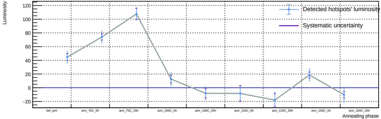
Sensor A1, T = 20\text{ C} , v_{\text{over}} = 7\text{ V} - Spot 44: luminosity vs phase
