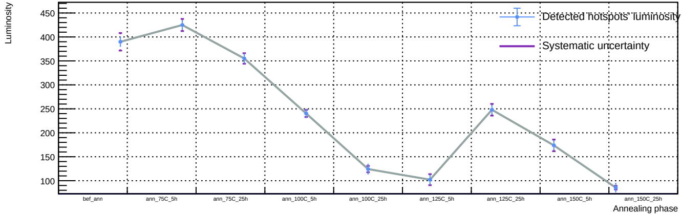
Sensor A1, T = 20\text{ C} , v_{\text{over}} = 7\text{ V} - Spot 45: luminosity vs phase
