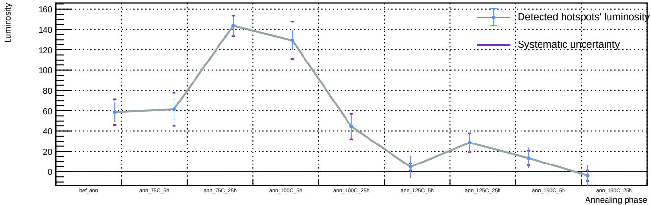
Sensor A1, T = 20\text{ C} , v_{\text{over}} = 7\text{ V} - Spot 47: luminosity vs phase
