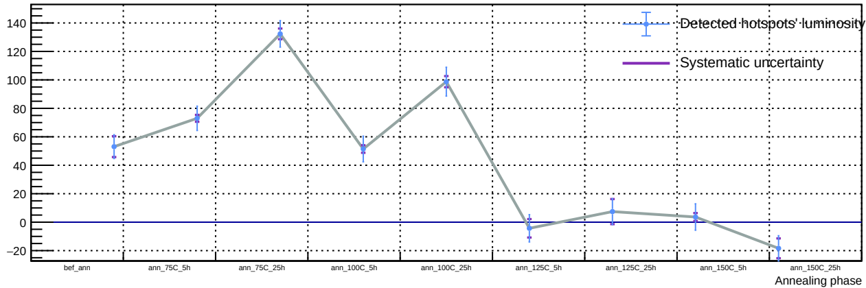
Sensor A1, T = 20\text{ C} , v_{\text{over}} = 7\text{ V} - Spot 53: luminosity vs phase
