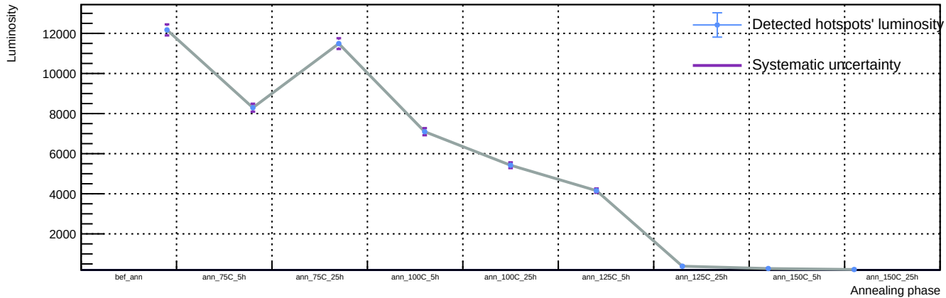
Sensor A1, T = 20\text{ C} , v_{\text{over}} = 7\text{ V} - Spot 54: luminosity vs phase
