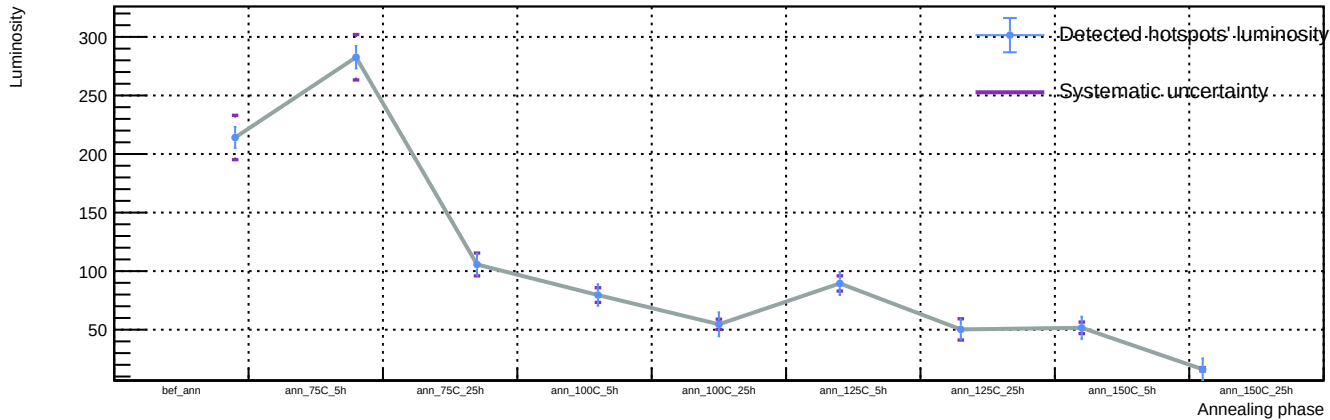
Sensor A1, T = 20\text{ C} , v_{\text{over}} = 7\text{ V} - Spot 65: luminosity vs phase
