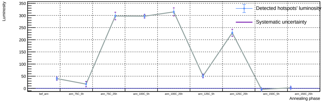
Sensor A1, T = 20\text{ C} , v_{\text{over}} = 7\text{ V} - Spot 66: luminosity vs phase
