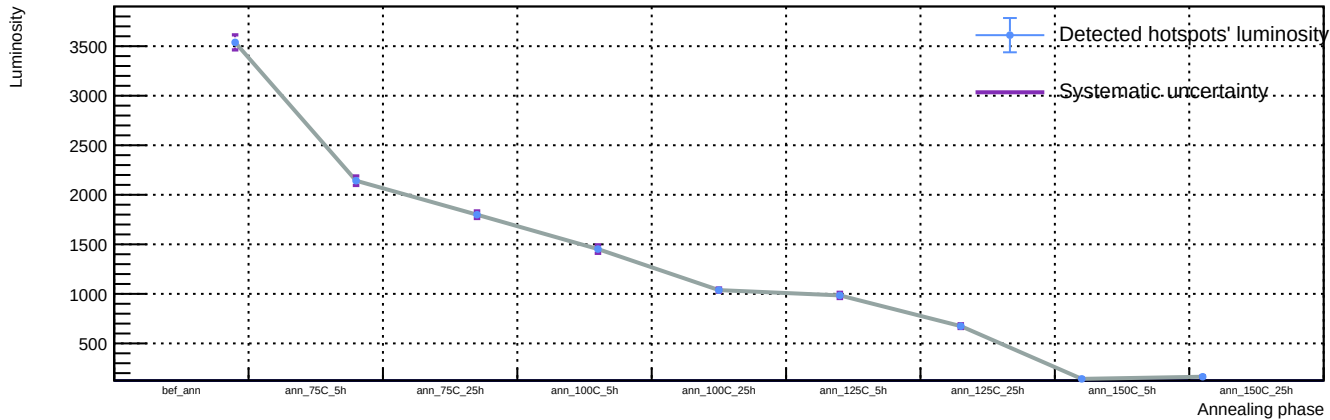
Sensor A1, T = 20\text{ C} , v_{\text{over}} = 7\text{ V} - Spot 67: luminosity vs phase
