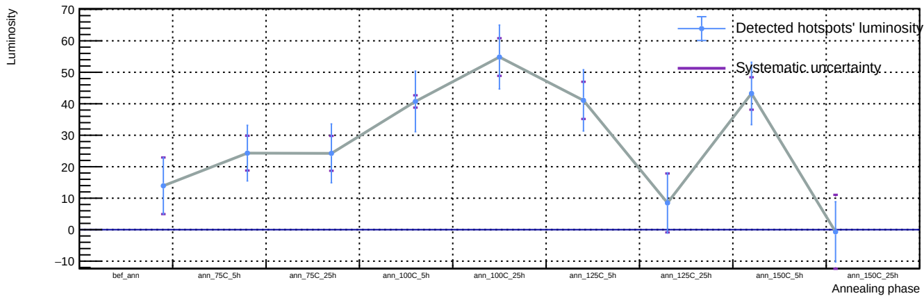
Sensor A1, T = 20\text{ C} , v_{\text{over}} = 7\text{ V} - Spot 68: luminosity vs phase
