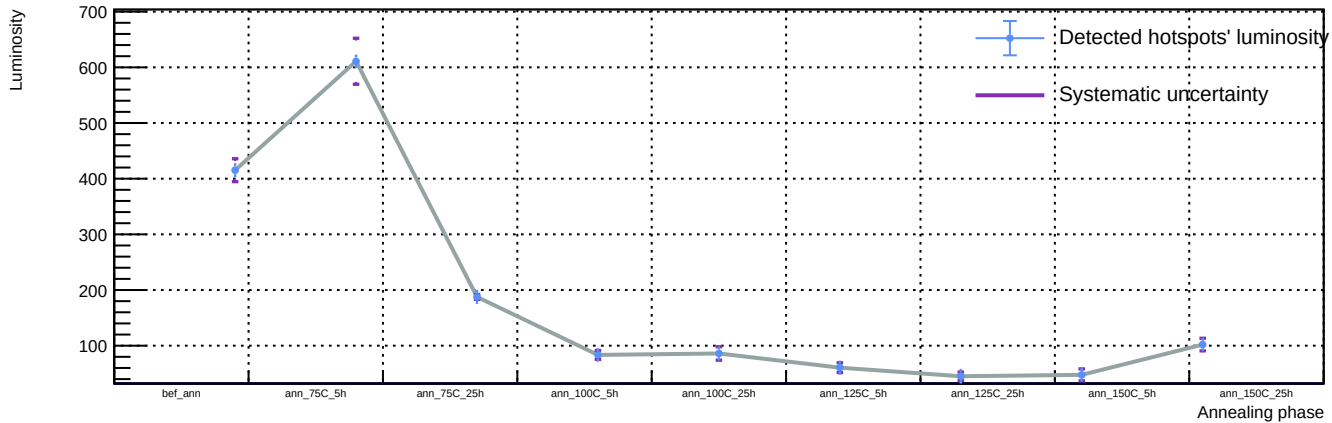
Sensor A1, T = 20\text{ C} , v_{\text{over}} = 7\text{ V} - Spot 69: luminosity vs phase
