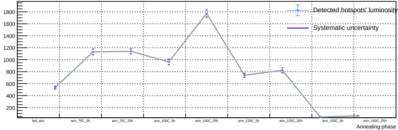
Sensor A1, T = 20\text{ C} , v_{\text{over}} = 7\text{ V} - Spot 7: luminosity vs phase
