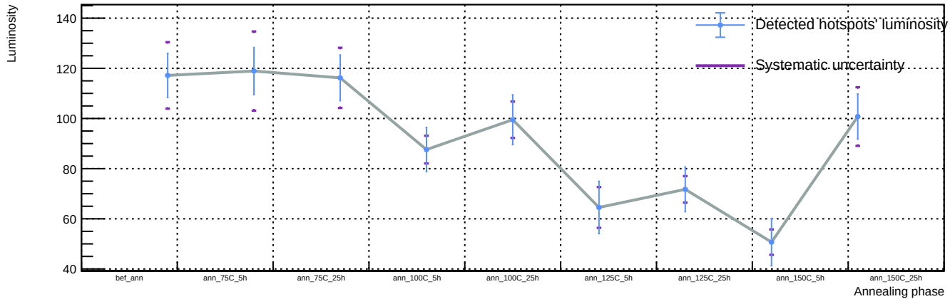
Sensor A1, T = 20\text{ C} , v_{\text{over}} = 7\text{ V} - Spot 70: luminosity vs phase
