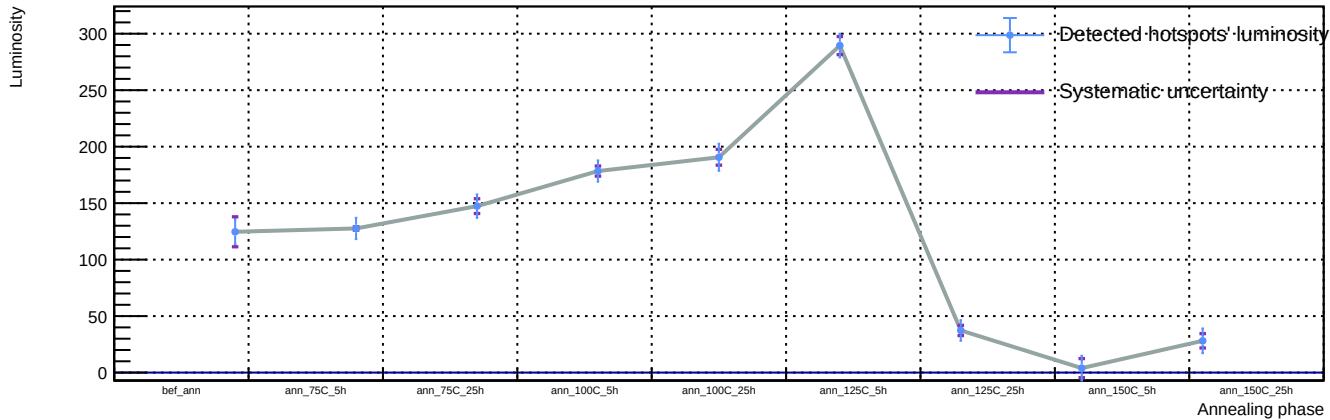
Sensor A1, T = 20\text{ C} , v_{\text{over}} = 7\text{ V} - Spot 71: luminosity vs phase
