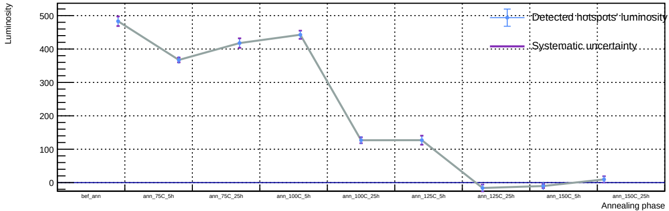
Sensor A1, T = 20\text{ C} , v_{\text{over}} = 7\text{ V} - Spot 72: luminosity vs phase
