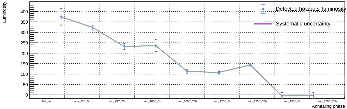
Sensor A1, T = 20\text{ C} , v_{\text{over}} = 7\text{ V} - Spot 75: luminosity vs phase
